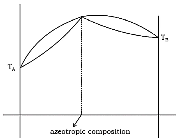
Boiling temperature - composition Diagram for solutions showing large negative deviations. (Maximum boiling azeotrope)
