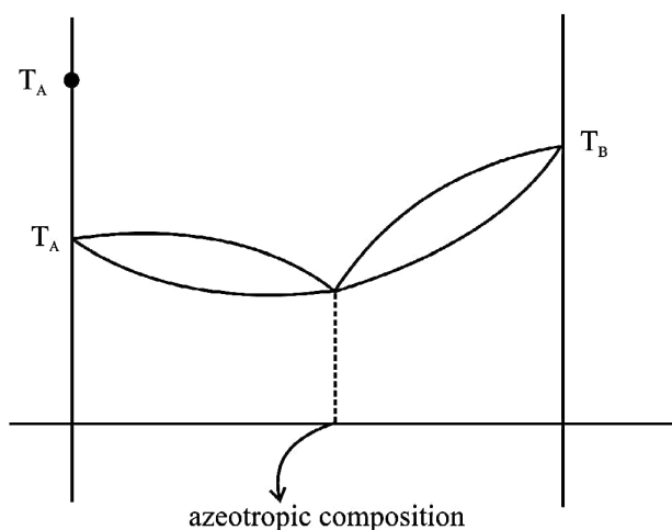
Boiling temperature - composition Diagram for solutions showing large positive deviations. (Minimum boiling azeotrope)
