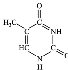
Thymine (T)
