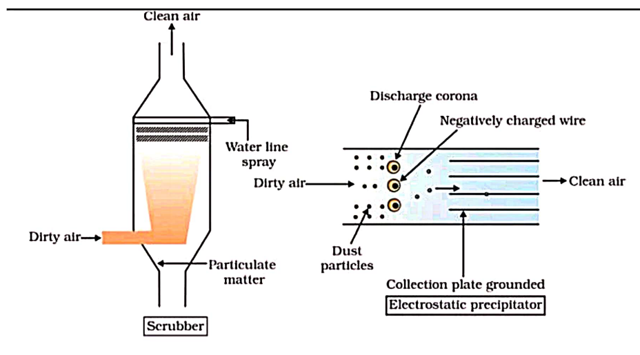
Electrostatic Precipitator
