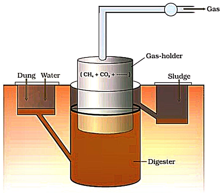
Fig.4. Gobar gas production
